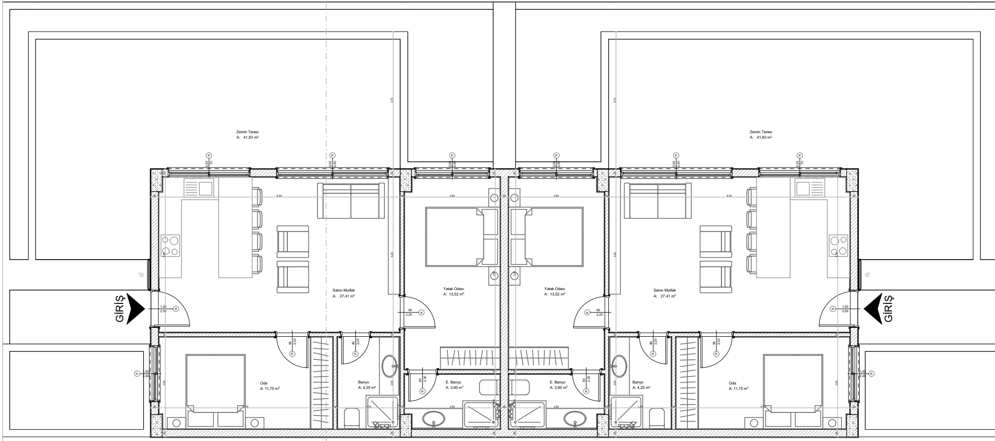
ZEMİN KAT PLAN
