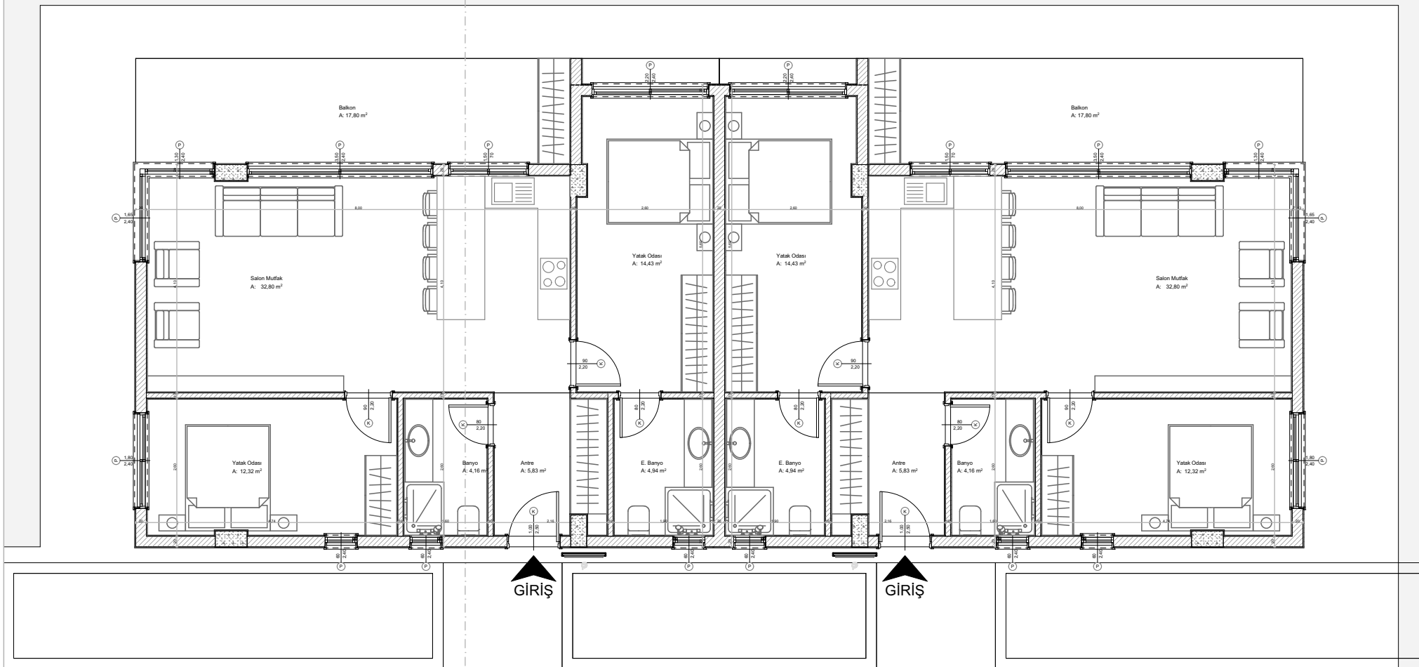
1.KAT PLAN
